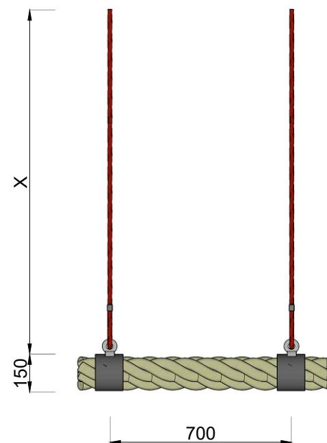
KUNUNURRA FRONT ELEVATION SCALE 1:20 @ A3
