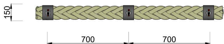
DERBY TOP VIEW SCALE 1:20 @ A3
